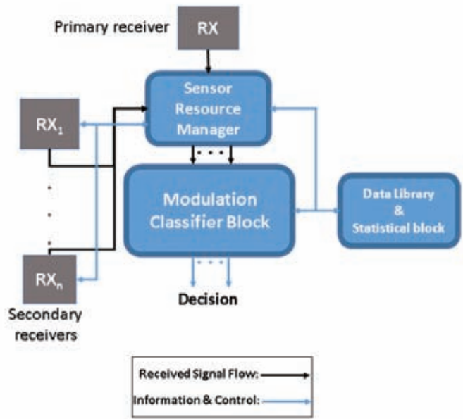
Fig. 1: Framework for automatic signal classification
