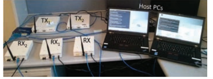
Fig. 6: Experimental setup
