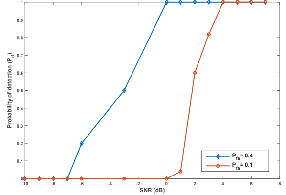
Fig. 7: FACT's probability of signal detection ( P_d ) vs SNR
