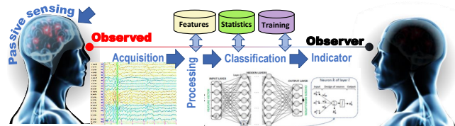
Fig. 1: Brain-Observer-Indicator framework.
