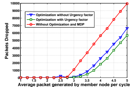
Figure 11: Packets dropped (SNR range: 1dB-15dB).
