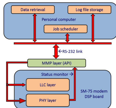
Figure 13: Communication architecture.
